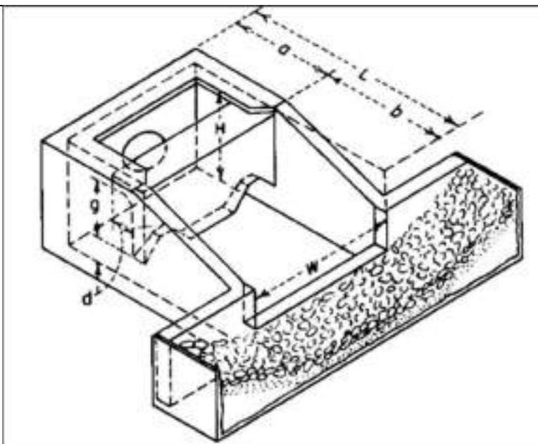
Figure 37: Concept design of effluent structure and stormwater control (SMEC, August 2025)
