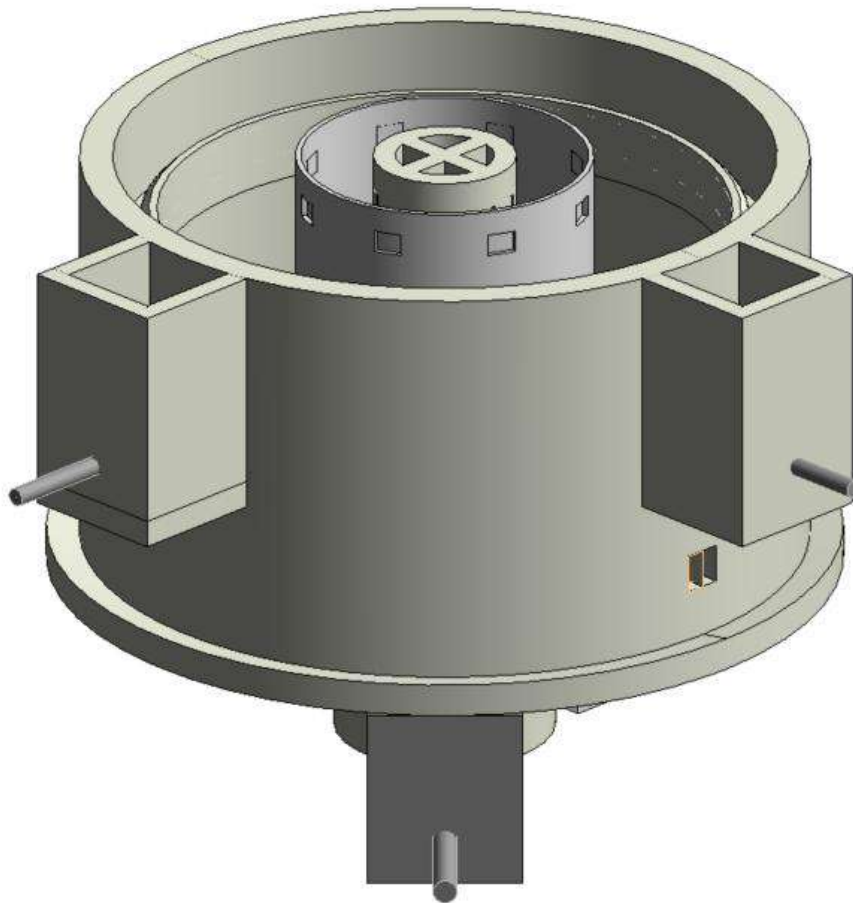
Figure 5-14 Clarifier
