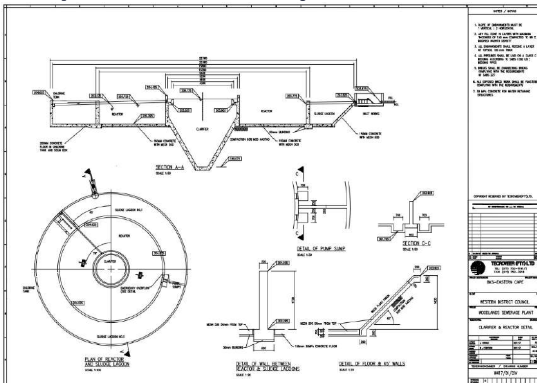
Figure 4-7 Woodlands WWTW Reactor and Clarifier detail
