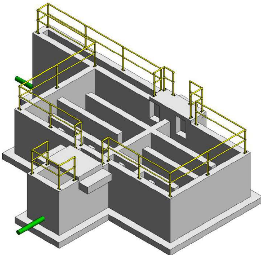
Figure 5-15 Chlorine Contact Tank
